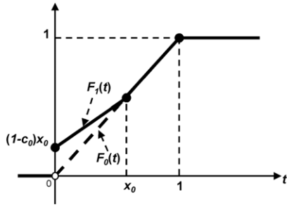
Fig. 2. The CDFs, F_0 and F_1 , of X_0 and X_1 under the null hypothesis.
