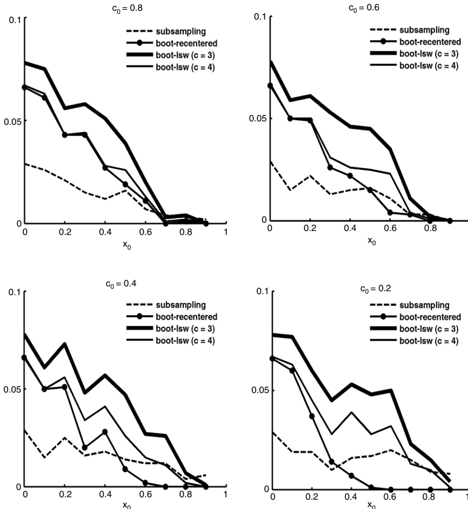
Fig. 3. The rejection probabilities under the null hypothesis: \alpha = 0.05 .
