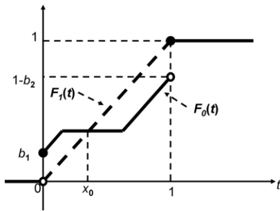
Fig. 4. The CDFs of X_0 and X_1 under the alternatives.
