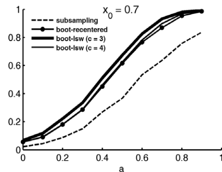
Fig. 5. The rejection probabilities under the alternatives: \alpha = 0.05 .
