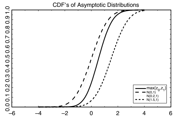
Fig. 1. The CDFs of Asymptotic Distributions of the Test Statistic T_N under the Null (N(0, 1)) and the Alternative Hypotheses (N(0.2, 1) and N(1.5, 1)) . The results show that the test is asymptotically biased against H_N for \delta = 0.2 .
